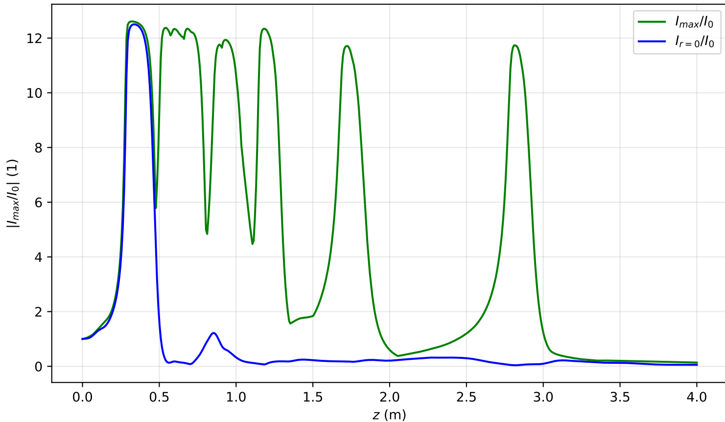
I_{max}(x=0, y=0, z)/I_0 , Pin=8.8Pcr, noisy input, artificial time
